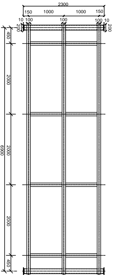
SKID - TOP VIEW
