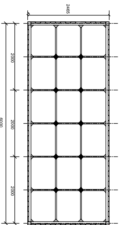
CEILING FRAME - TOP VIEW
