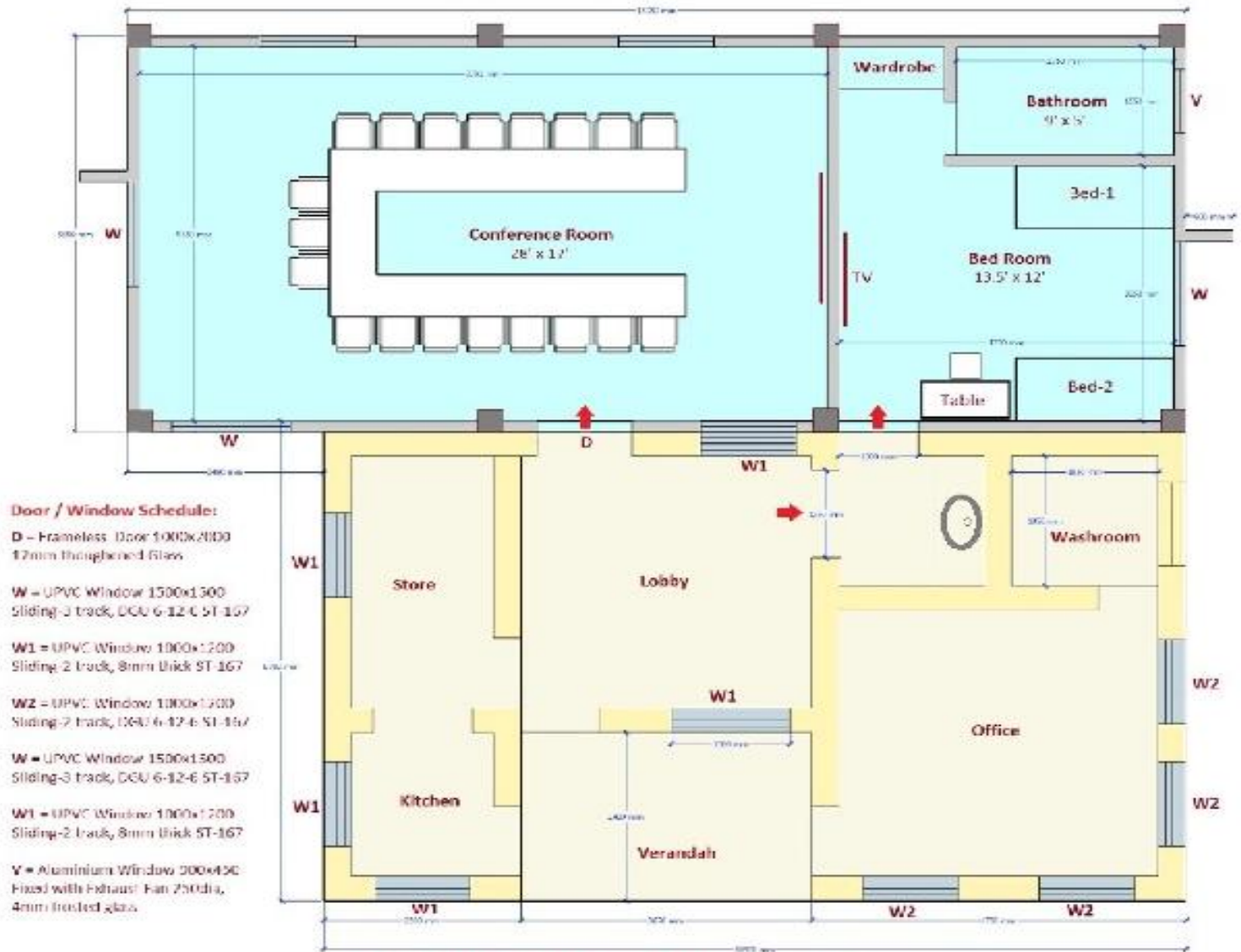
PROPOSED HAMIRA ROOM EXTENSION
