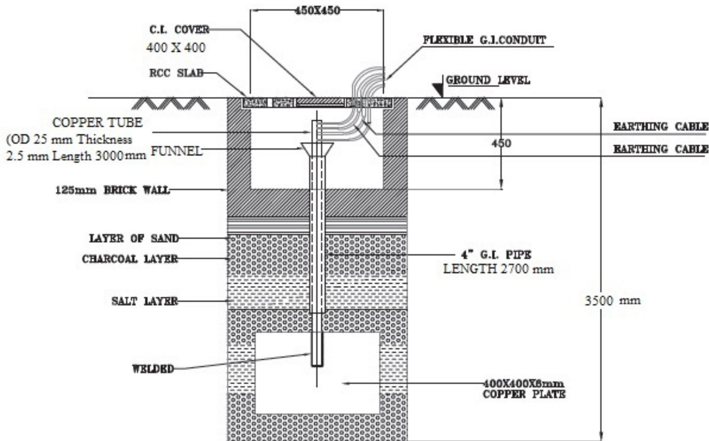
DETAIL OF EARTH PIT (TYPICAL)
